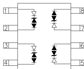
SO-8 outline
