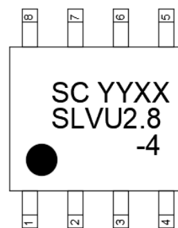
YYXX= Date Code Dot denotes Pin1
